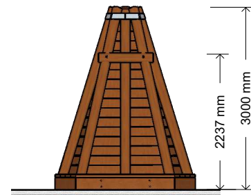
2 Front View Scale: NTS
