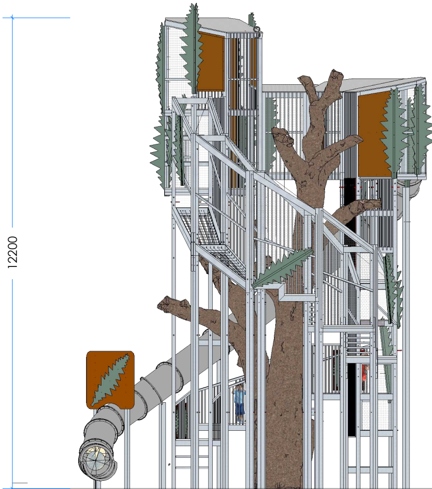
2 Elevation Scale 1:100
