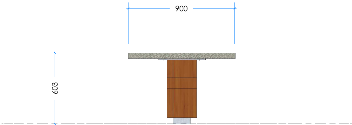
2 Elevation Scale 1:20
