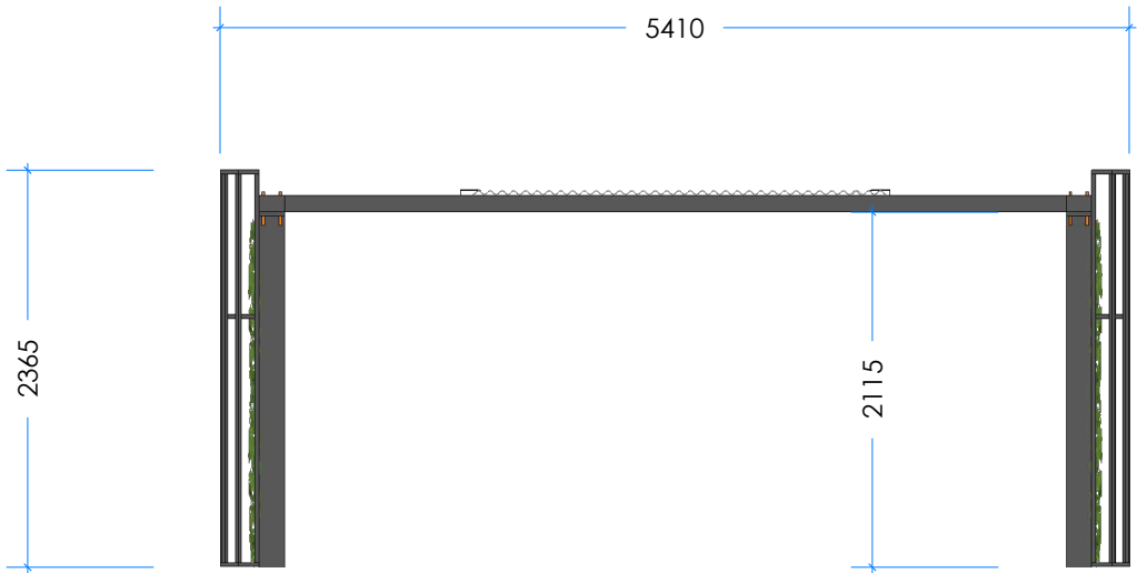
2 Elevation Scale 1:50
