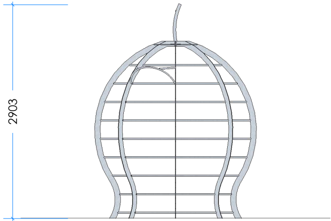
2 Elevation Scale 1:50
