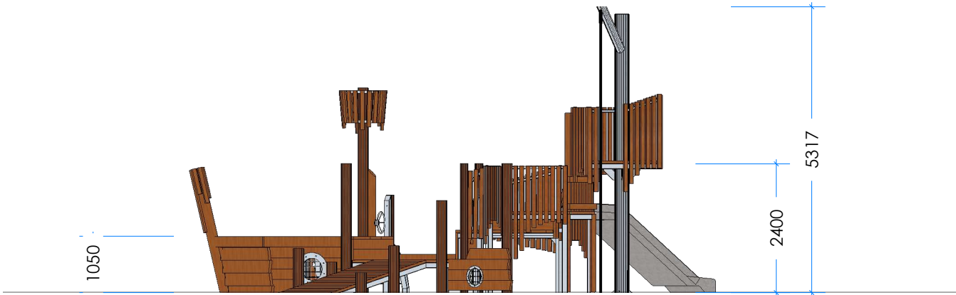
2 Elevation Scale 1:100
