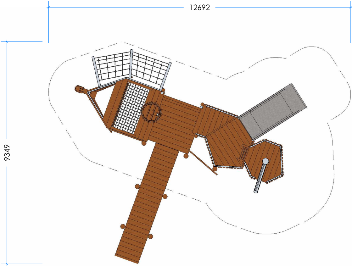
3 Top Scale 1:100
