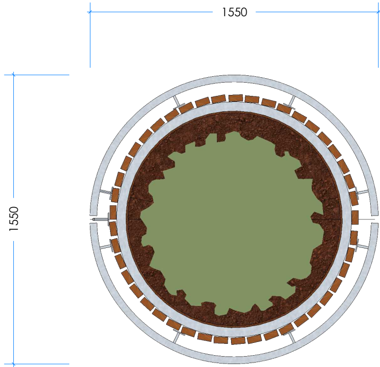
3 Top Scale 1:20
