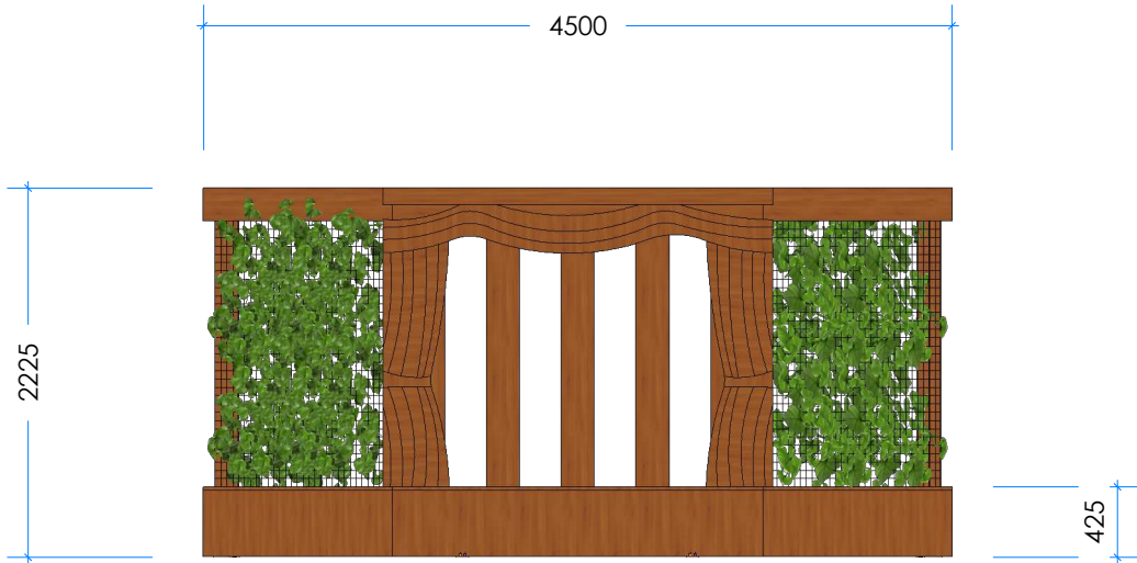
2 Elevation Scale 1:50
