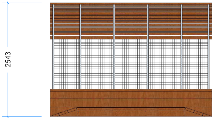
2 Elevation Scale 1:50
