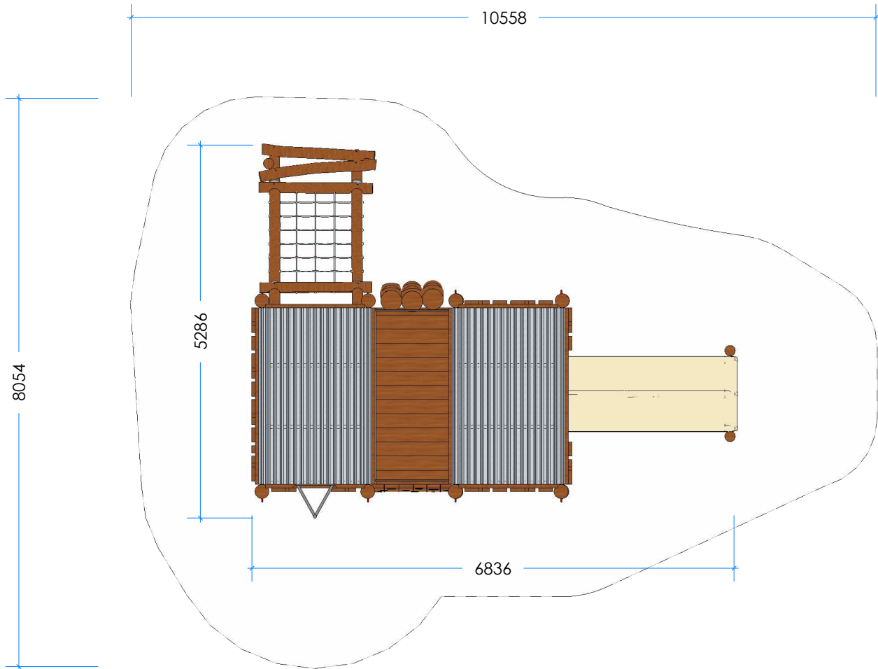
3 Top Scale 1:75
