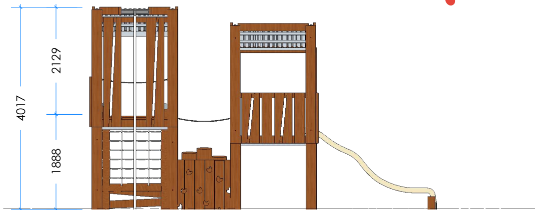
2 Elevation Scale 1:75
