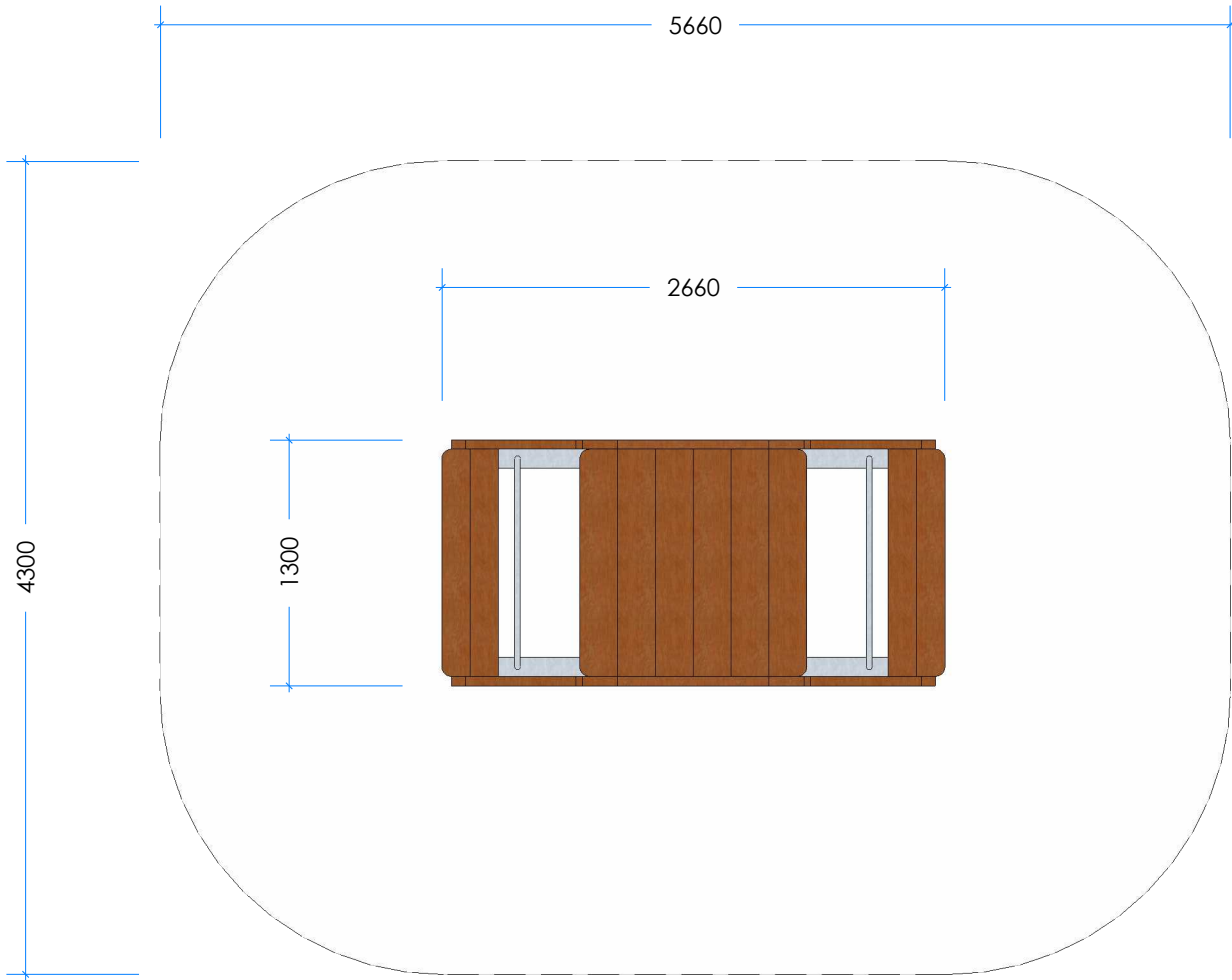
3 Top Scale 1:40
