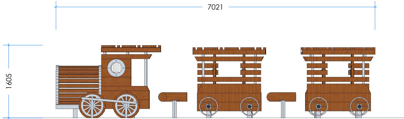
2 Elevation Scale 1:50
