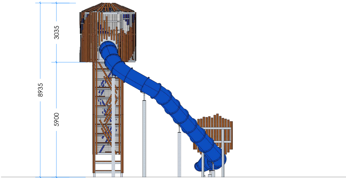
2 Elevation Scale 1:100
