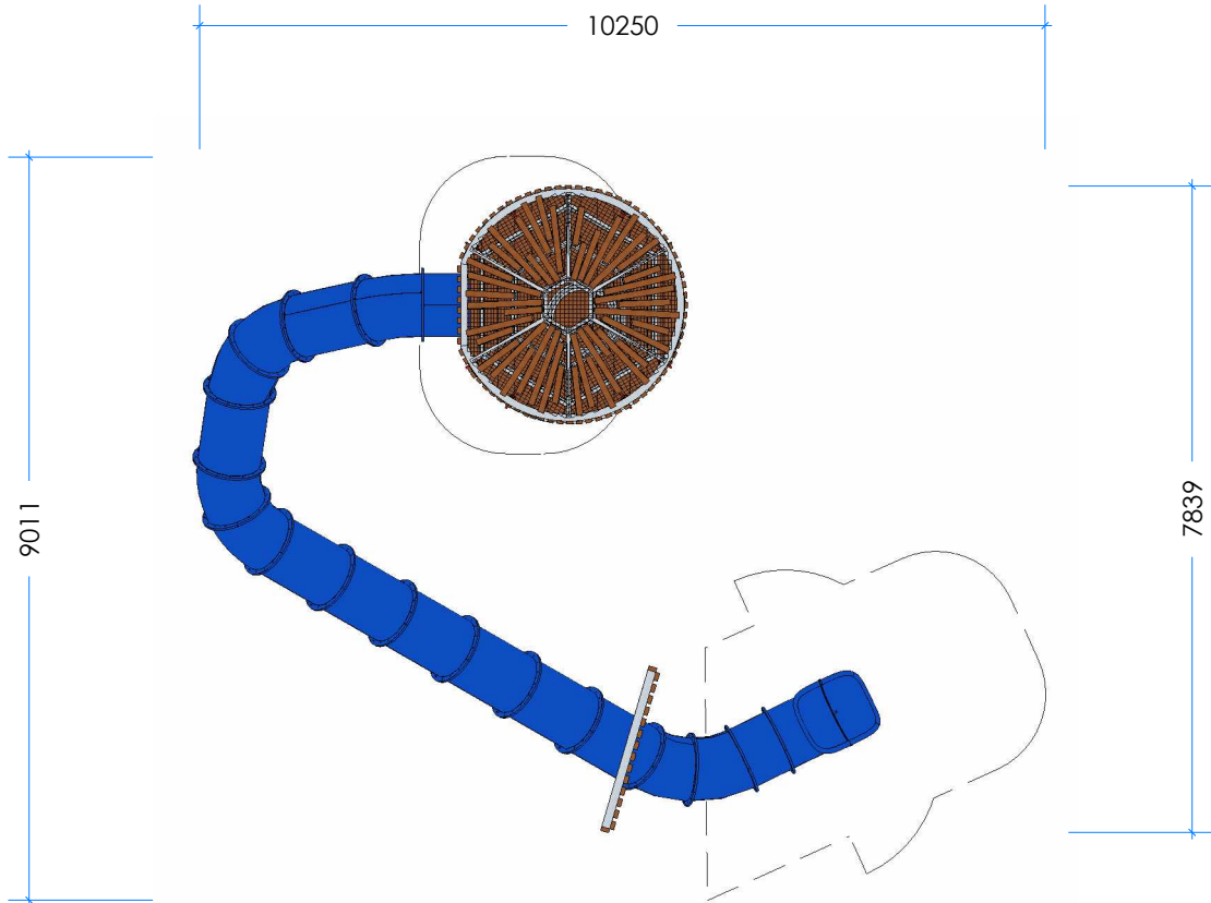
3 Top Scale 1:100
