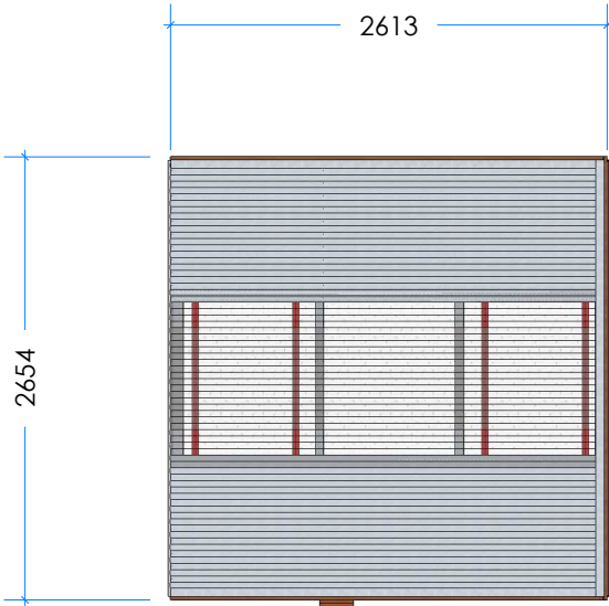
3 Top Scale 1:50
