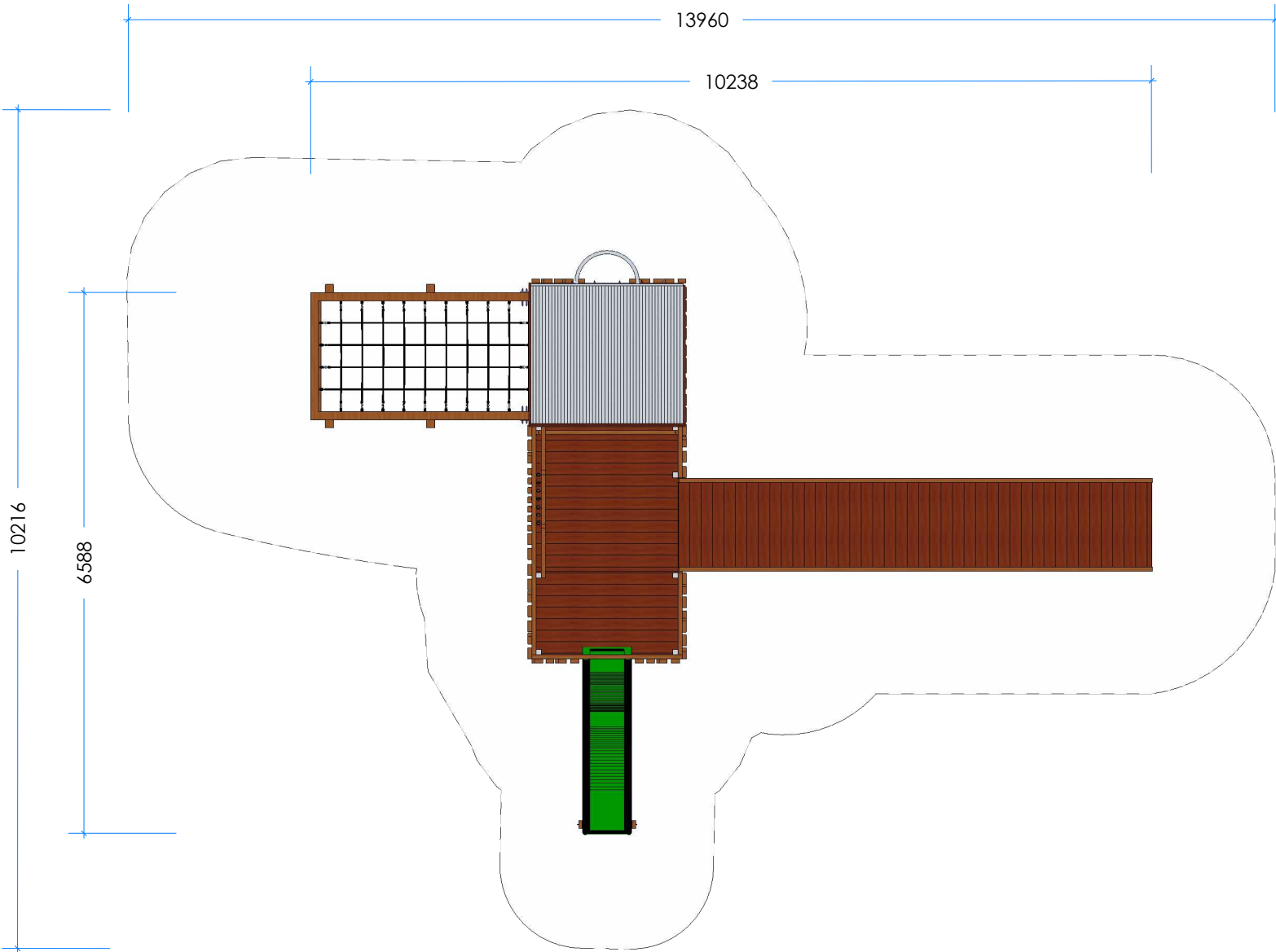
3 Top Scale 1:75
