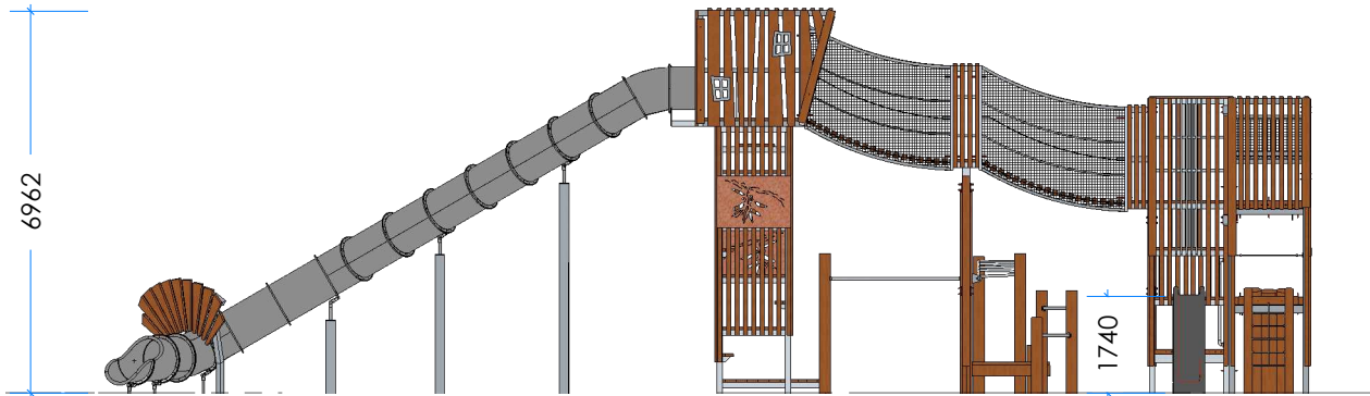
2 Elevation Scale 1:150
