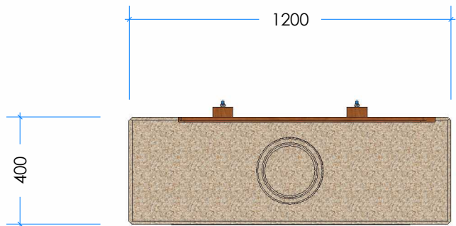
3 Top Scale 1:20
