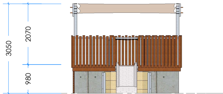
2 Elevation Scale 1:75
