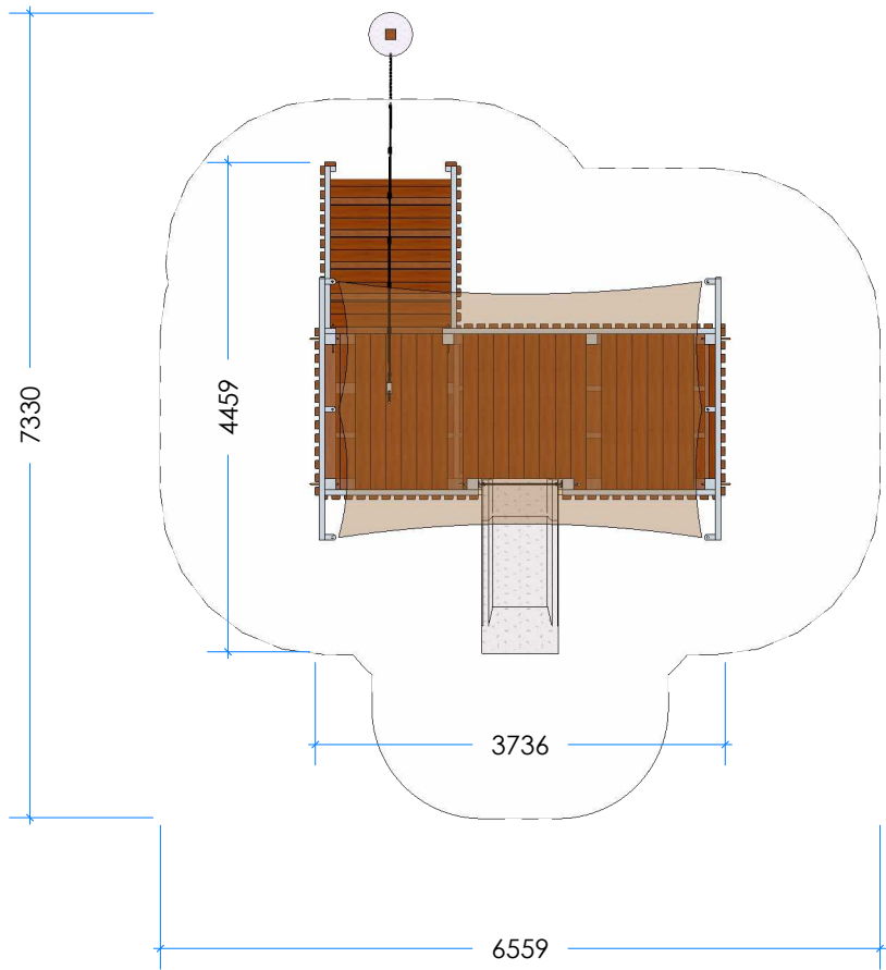
3 Top Scale 1:75
