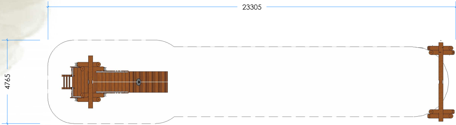
3 Top Scale 1:125
