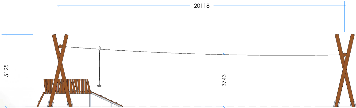
2 Elevation Scale 1:125
