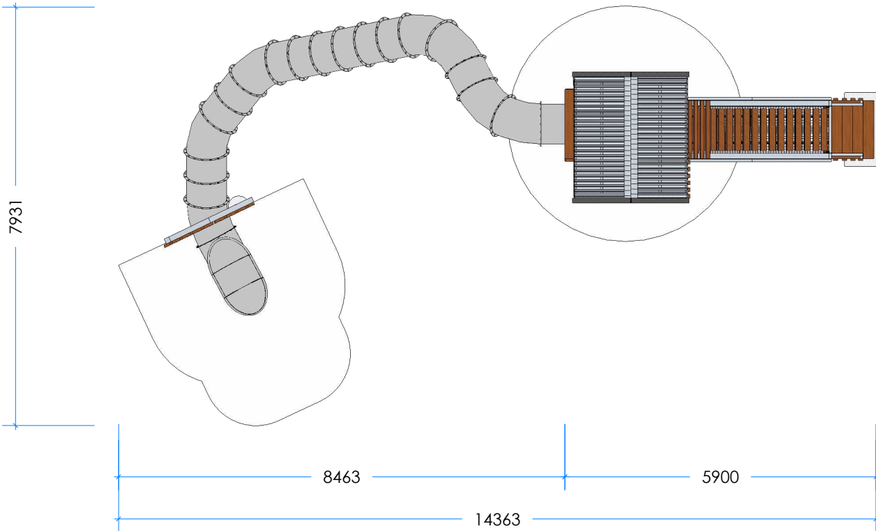
3 Top Scale 1:100
