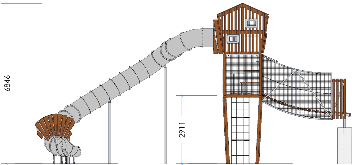
2 Elevation Scale 1:100
