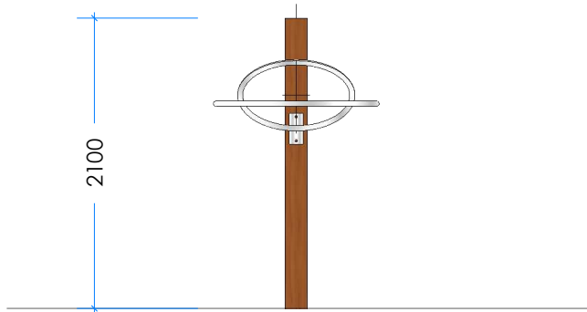
2 Elevation Scale 1:50
