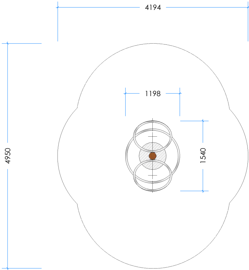
3 Top Scale 1:50
