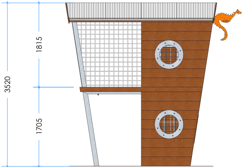
2 Elevation Scale 1:50
