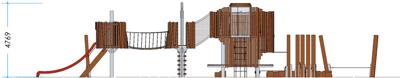
2 Elevation Scale 1:150
